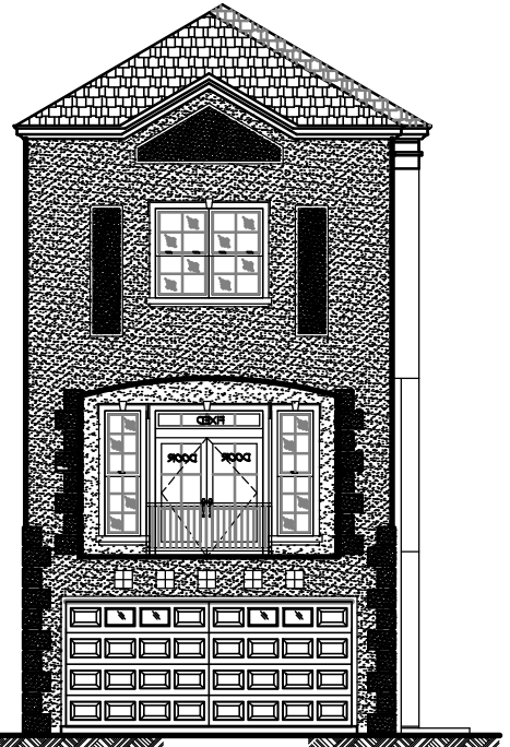
FRONT ELEVATION
