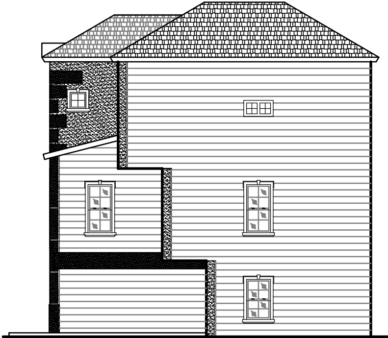
SIDE ELEVATION
