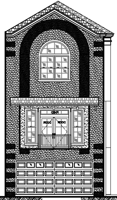
FRONT ELEVATION
